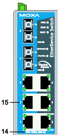
Front Panel View
