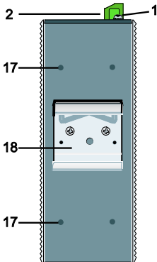
Rear Panel View
