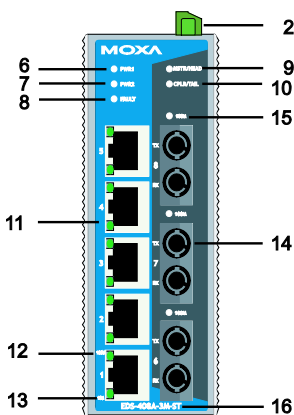
EDS-408A-3M-ST Front Panel View
