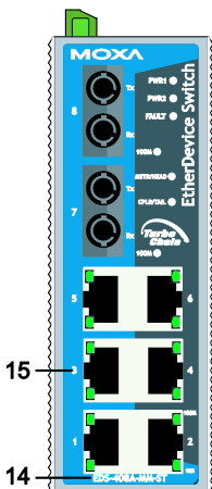
EDS-408A-MM-ST Front Panel View
